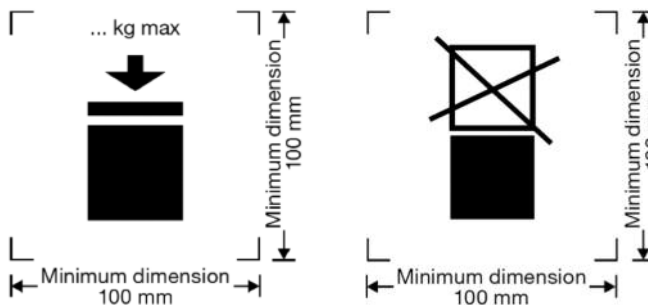
Left: Symbol for IBCs capable of being stacked, with the maximum stack weight indicated
