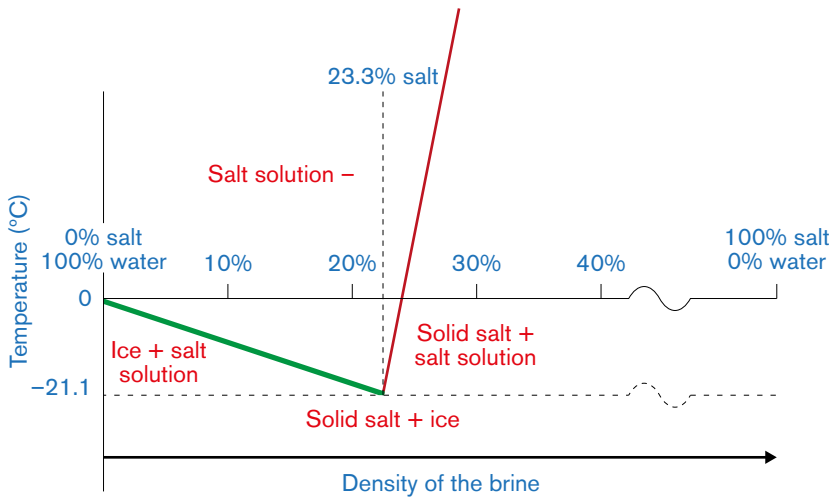
Figure 38.5: Lowering of freezing point of brine.
