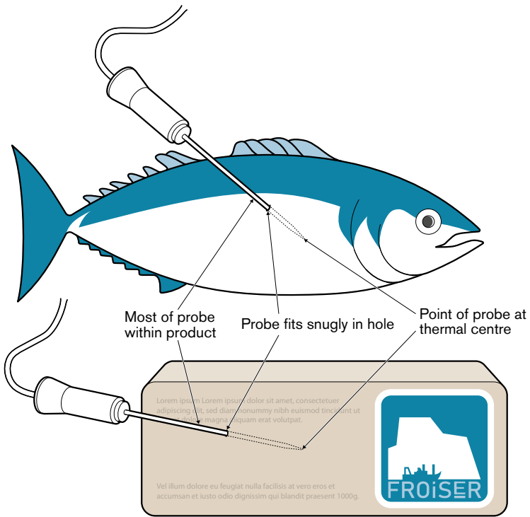
Figure 38.10: Inserting temperature probe into frozen fish or block of fish.
