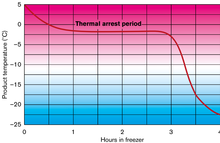
Figure 38.4: Freezing curve of fish initially at 5°C.
