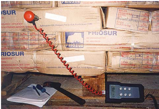
Figure 38.12: Measuring temperature within a carton.
