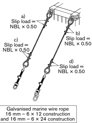
Figure 54.9: Soft eyes – some other representative slip loads.
