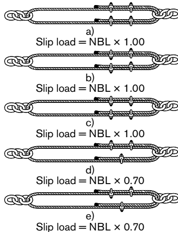
Figure 54.11: Half-double grommets – some other representative slip loads.
