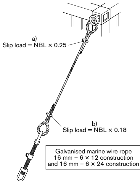
Figure 54.10: Soft eyes – UNSAFE application of Bulldog clips.
