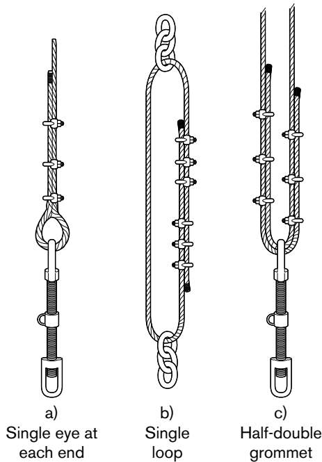
Figure 54.7: Configurations tested.
