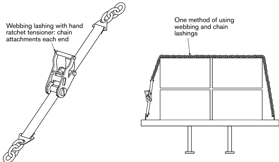
Figure 54.14: Webbing.
