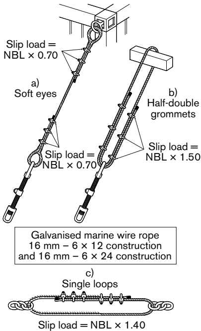
Figure 54.8: Correct application of Bulldog grips.
