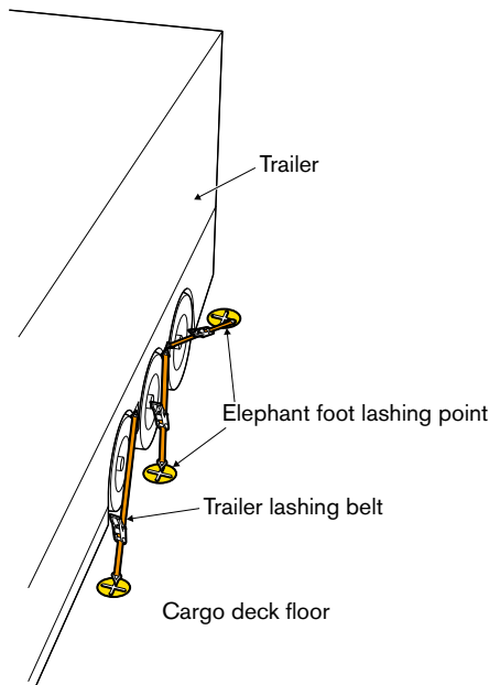
Figure 54.3: Lashing of cargo RoRo.
