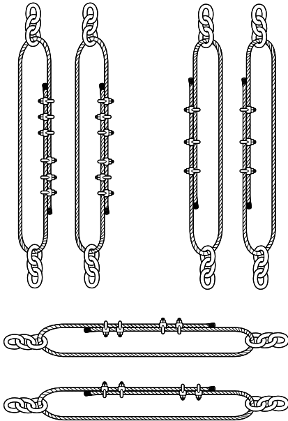
Figure 54.12: Single loops – some other representative slip loads.
