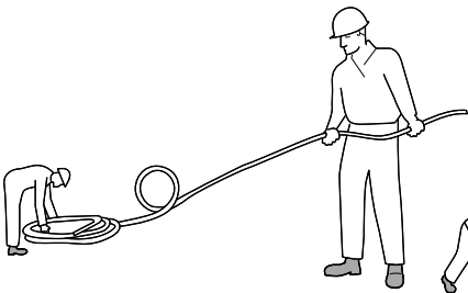
Unreeling: incorrect method
