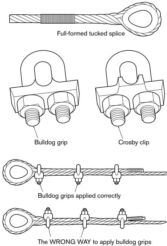
Figure 54.6: Grips and clips.
