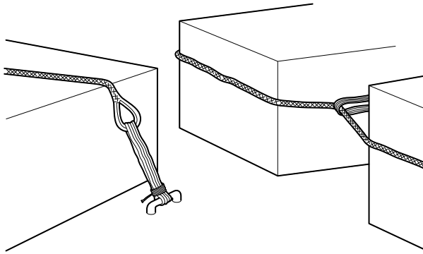
Figure 54.15: Tightening rope lashings.
