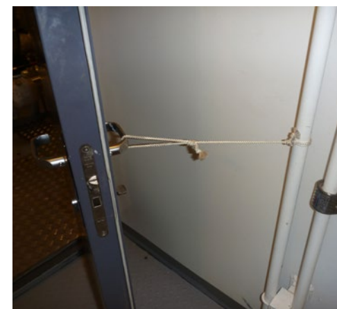
X Self-closing doors in fire division bulkheads should not be secured in the open position when not in use.
